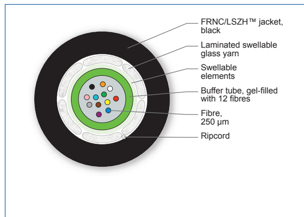
Cross Section of Order Number: 012TEU-13198A2G
