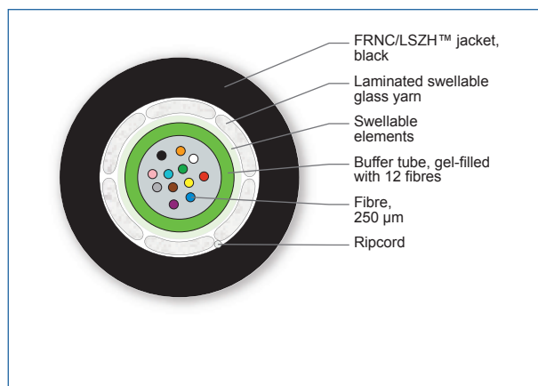
Cross Section of Order Number: 012TEU-13138A2G
