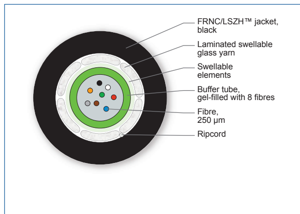
Cross Section of Order Number: 008TEU-13138A2G
