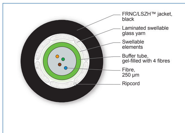
Cross Section of Order Number: 004TEU-13138A2G
